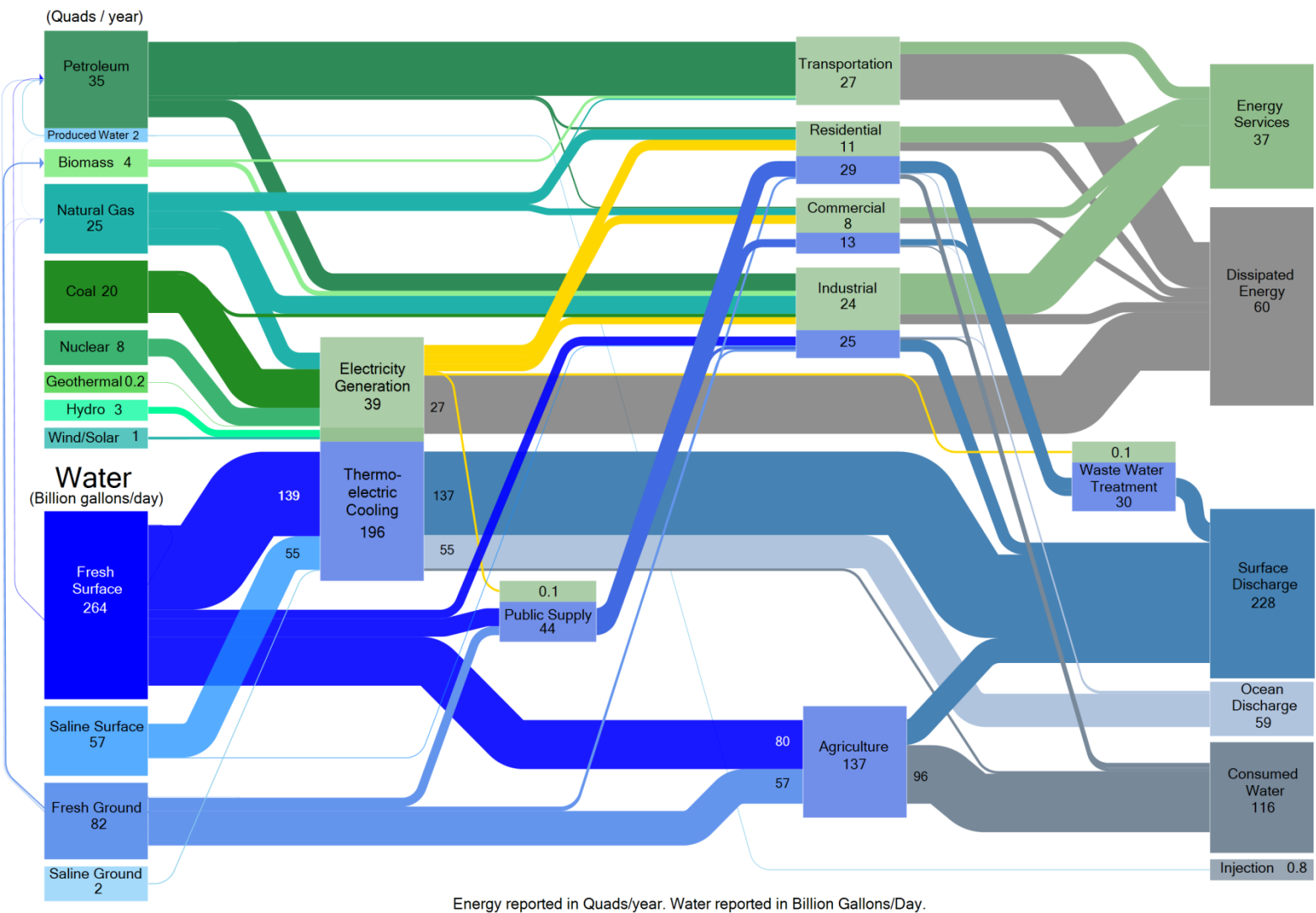
Figure 2.1. Hybrid Sankey diagram of interconnected U.S. water and energy flows in 2011. Source: See Appendix A for data sources and calculations
